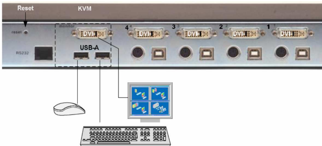
Figure 3. Local KVM Console Installation
