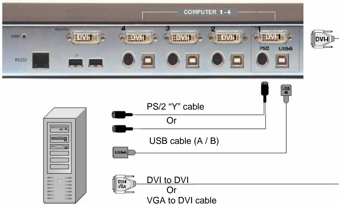
Figure 4. Video source installation
